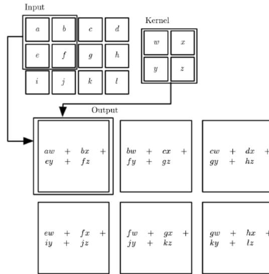
Figure 2.3.: Image from [GBC16]. In the top left the values a, b, e and f are multiplied with the values from the kernel. The values are added and produce one output value. This is repeated for the input positions for all possible kernel positions of the kernel being completely in the image.
